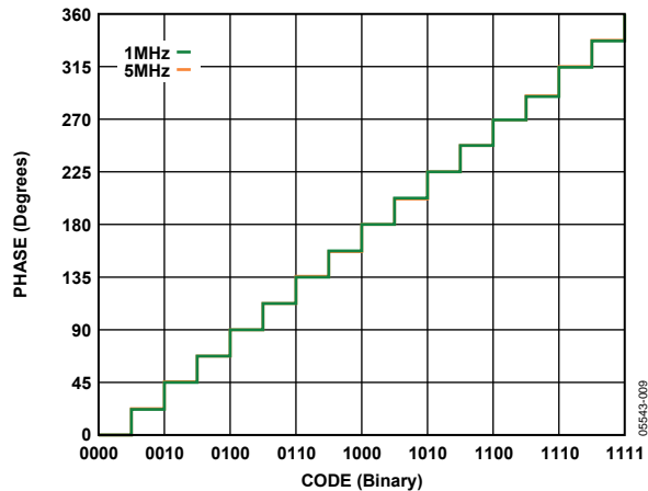
Figure 9. Phase of CH2 with Respect to CH1 vs. Code, at 1 MHz and 5 MHz
