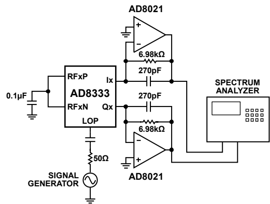
Figure 47. Noise Test Circuit
