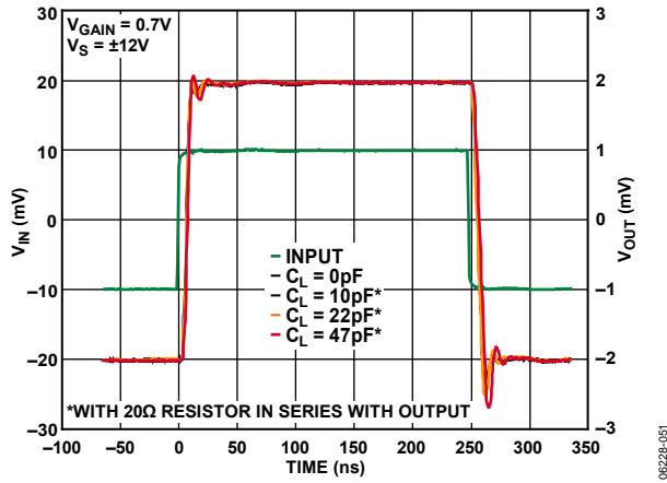
Figure 51. Large Signal Pulse Response for Various Values of Load Capacitance Using \pm 12\text{V} Power Supplies
