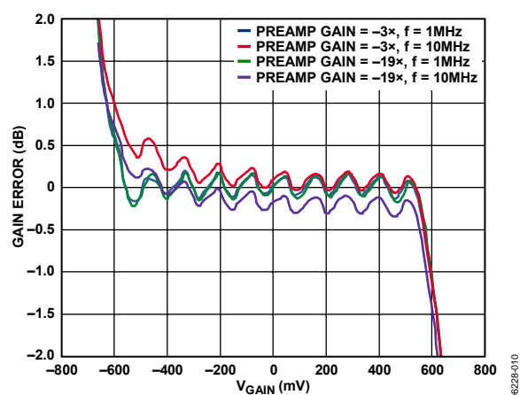
Figure 10. Gain Error vs. V_{\text{GAIN}} at 1 MHz and 10 MHz and for Inverting Preamp Gains of -3x and -19x
