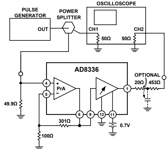
Figure 65. Pulse Response
