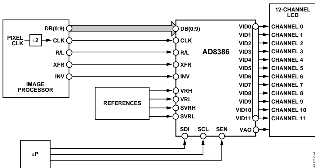
Figure 11. 12-Channel System
