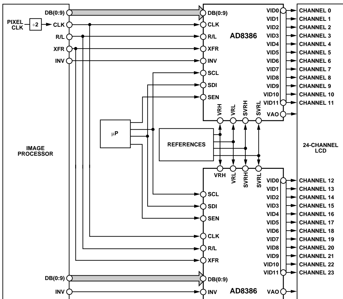
Figure 12. 24-Channel System
