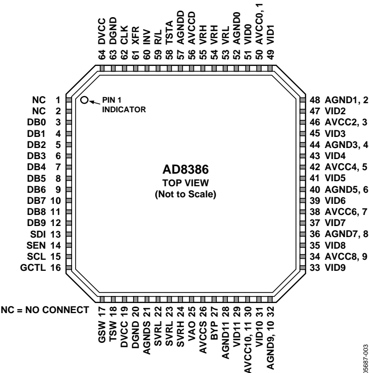
Figure 3. 64-Lead LFCSP_VQ Pin Configuration
