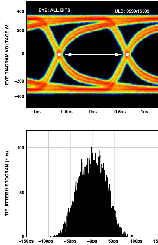
Figure 61. Data Eye for LVDS Outputs in ANSI Mode with 100 \Omega Termination on and Trace Lengths Greater than 24 Inches on Standard FR-4
