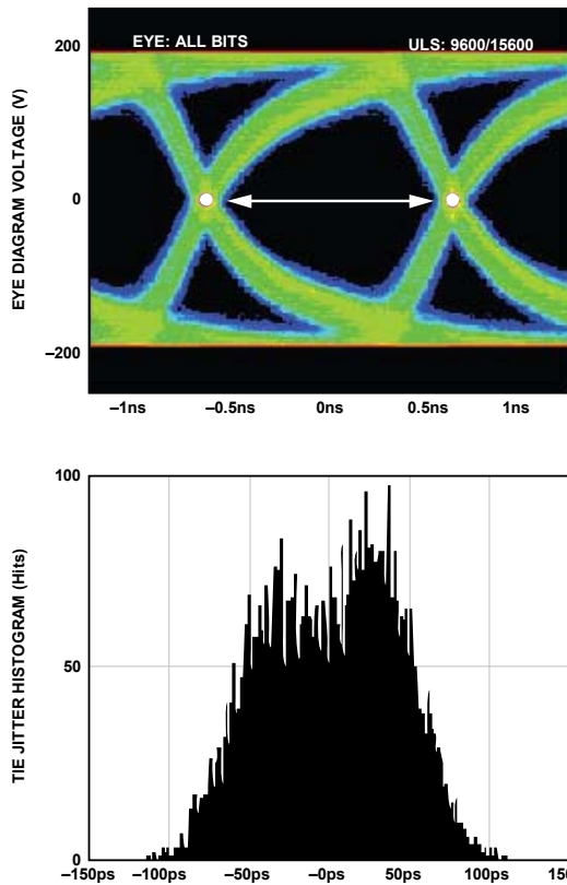
Figure 60. Data Eye for LVDS Outputs in ANSI Mode with Trace Lengths Greater than 24 Inches on Standard FR-4
