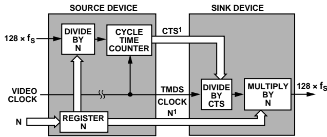
Figure 7. N and CTS for Audio Clock
