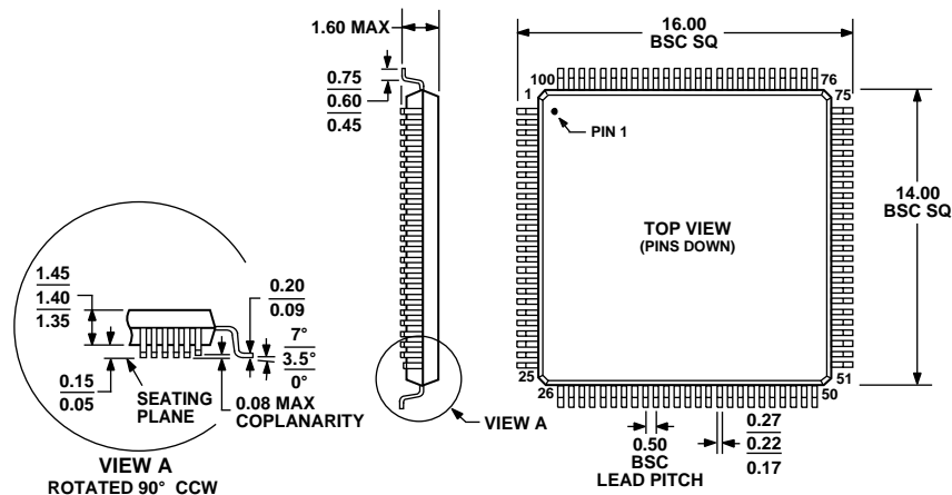
Figure 19. 100-Lead Low Profile Quad Flat Package [LQFP] (ST-100) Dimensions shown in millimeters
