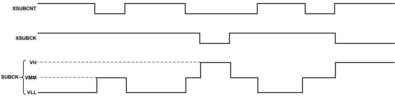
Figure 64. XSUBCK, XSUBCNT, and SUBCK Output Polarities
