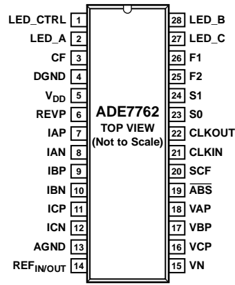
Figure 4. Pin Configuration
