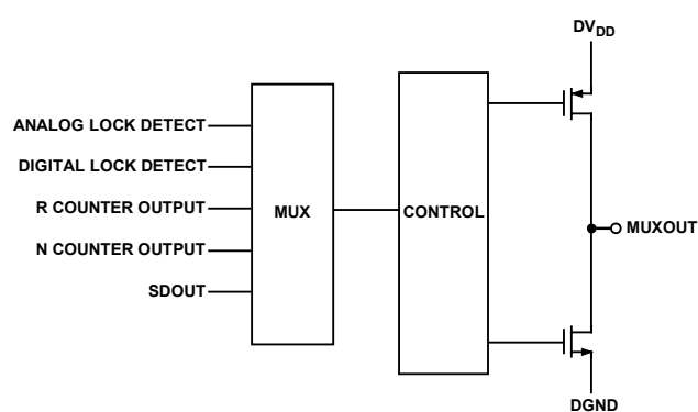
Figure 15. MUXOUT Circuit
