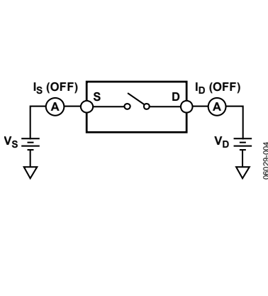
Figure 23. Off Leakage
