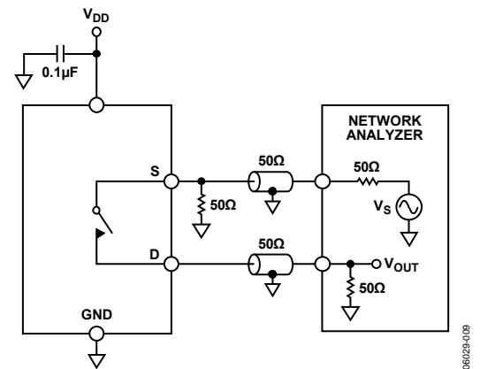
Figure 26. Off Isolation
