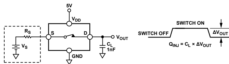
Figure 30. Charge Injection
