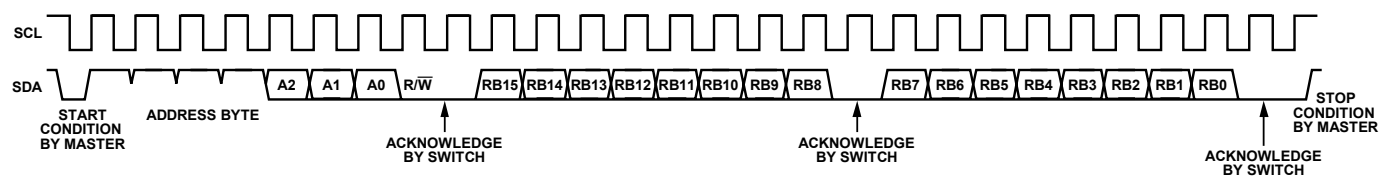
Figure 32. ADG795A/ADG795G Read Operation
