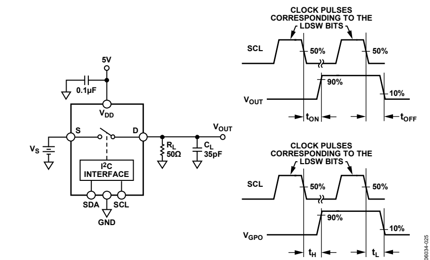
Figure 28. Switching Times
