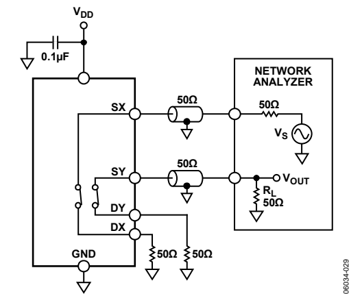
Figure 27. Channel-to-Channel Crosstalk
