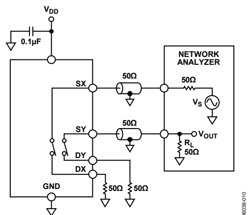
Figure 23. Channel-to-Channel Crosstalk
