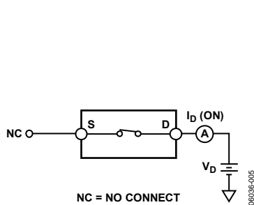
Figure 19. Off Leakage
