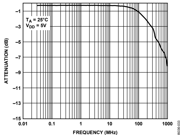
Figure 14. Bandwidth
