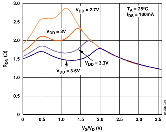
Figure 4. On Resistance vs. V_S (V_D) ; V_{DD} = 2.7 V to 3.6 V
