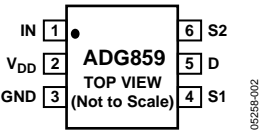
Figure 2. 6-Lead SOT-66 Pin Configuration
