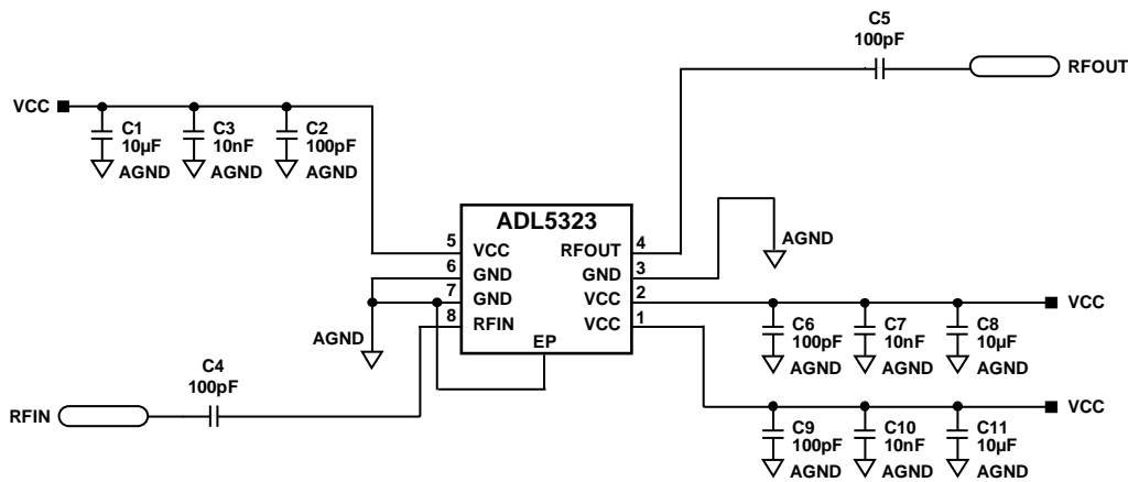
Figure 16. Basic Connections
