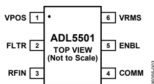
Figure 3. Pin Configuration
