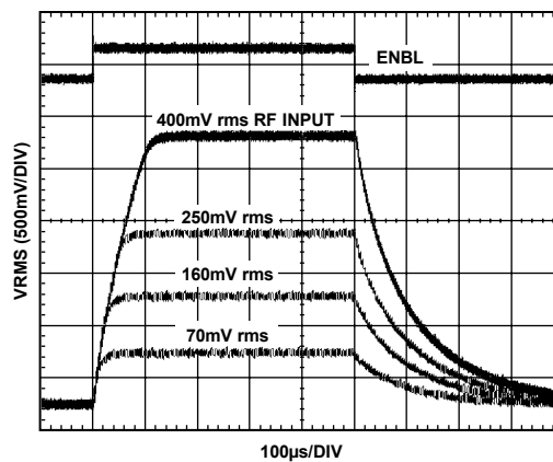
Figure 38. Output Response to Enable Gating at Various RF Input Levels, Supply 3 V, Frequency 900 MHz, C_{FLTR} = \text{Open} , C_{OUT} = 0.1\text{ }\mu\text{F} , R_{OUT} = 1\text{ k}\Omega
