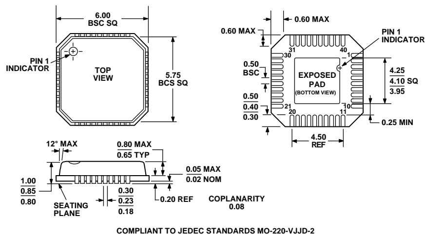
Figure 51. 40-Lead Lead Frame Chip Scale Package [LFCSP_VQ] 6 x 6 mm Body, Very Thin Quad (CP-40) Dimensions shown in millimeters
