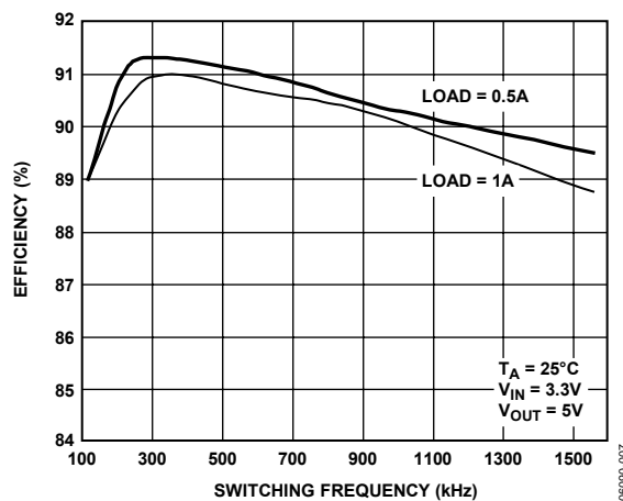
Figure 8. Efficiency vs. Switching Frequency
