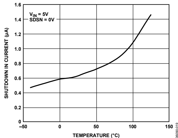
Figure 20. Shutdown IN Current vs. Temperature
