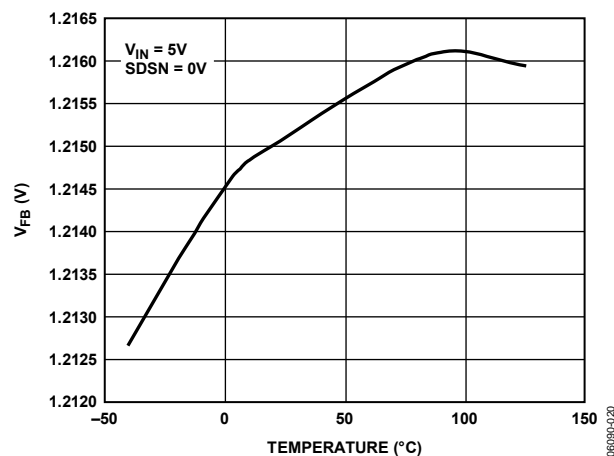
Figure 21. FB Voltage vs. Temperature
