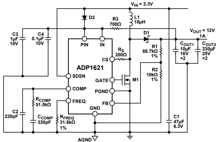
Figure 34. Bootstrapped Application Circuit for V_{OUT} > 5.5V
