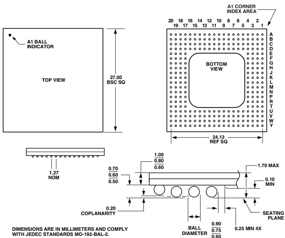
Figure 38. 256-Lead SBGA, Thermally Enhanced (BP-256)
