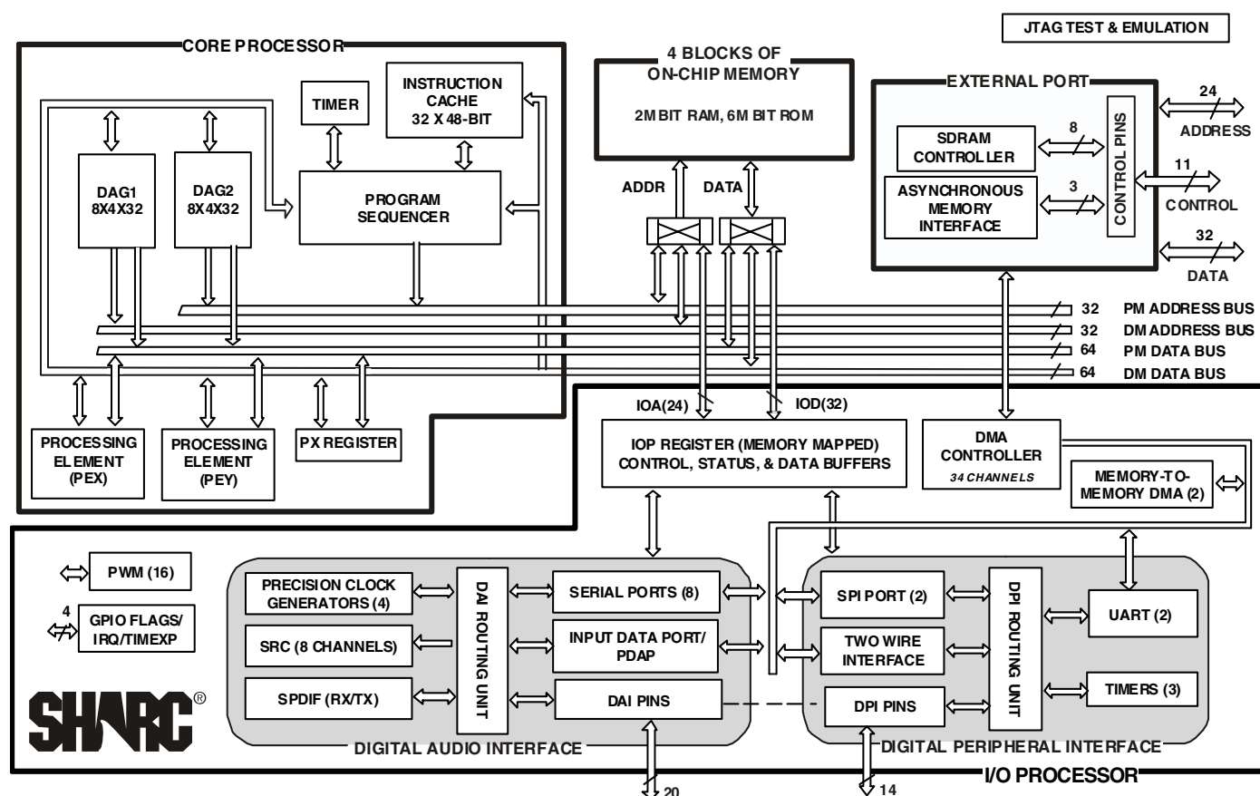
Figure 1. Functional Block Diagram – Processor Core
