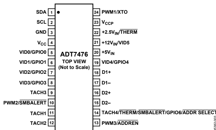
Figure 3. Pin Configuration
