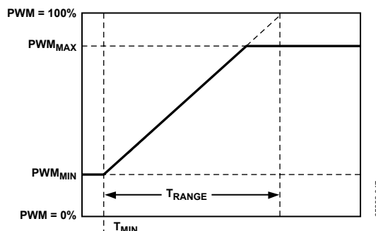
Figure 46. T RANGE
