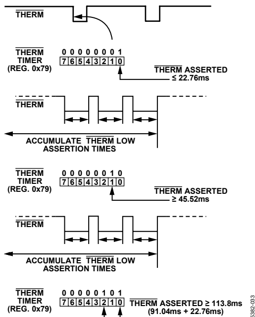
Figure 32. Understanding the \overline{\text{THERM}} Timer
