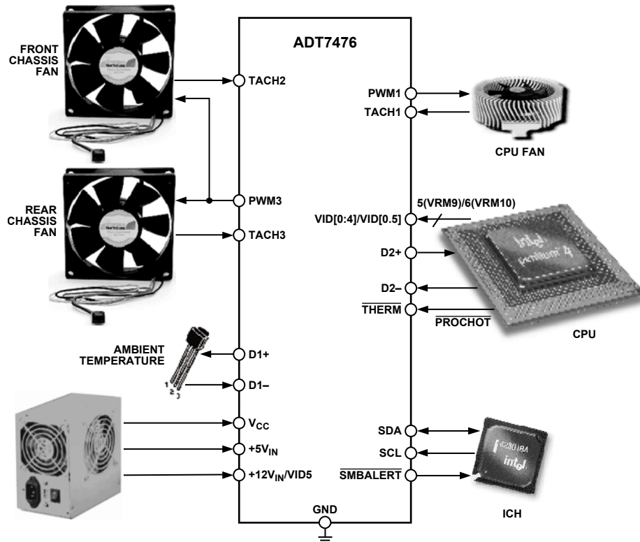
Figure 49. Recommended Implementation 1
