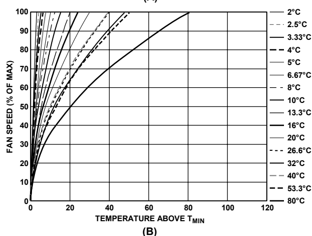
Figure 61. T_{\text{RANGE}} Vs. Actual Fan Speed (Not PWM Drive) Profile
