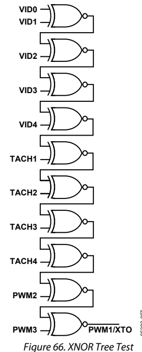
Figure 66. XNOR Tree Test
