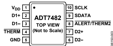
Figure 3. Pin Configuration
