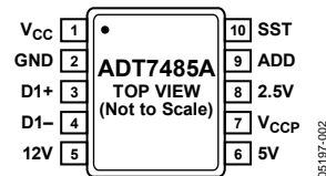
Figure 2. 10-Lead MSOP
