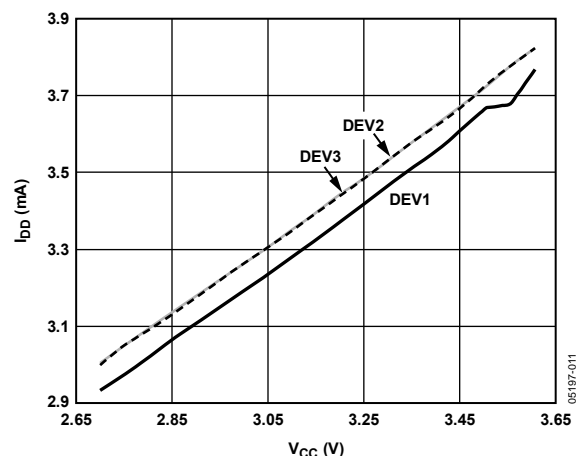
Figure 7. Supply Current vs. Voltage
