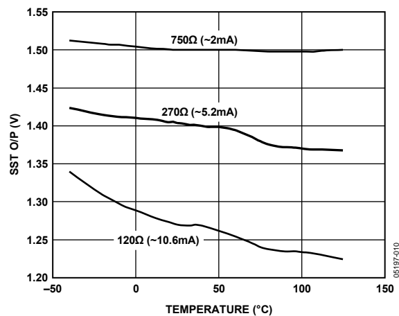
Figure 6. SST O/P Level vs. Temperature
