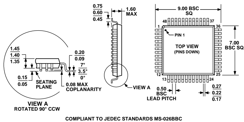
COMPLIANT TO JEDEC STANDARDS MS-026BBC Figure 10. 48-Lead Low Profile Quad Flat Package [LQFP] (ST-48) Dimensions shown in millimeters
