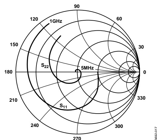
Figure 19. Input and Output Reflection Coefficients, S_{11} and S_{22} , Z_o = 100\ \Omega Differential
