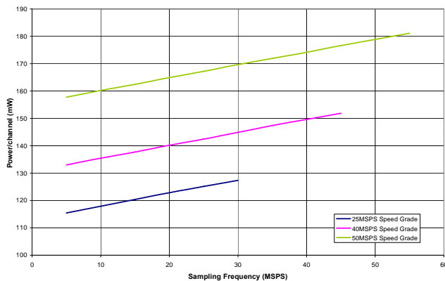
Figure 53. Power per Channel vs. f_{\text{SAMPLE}} for f_{\text{IN}} = 7.5 MHz
