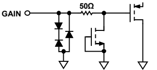
Figure 15. Equivalent GAIN Input Circuit
