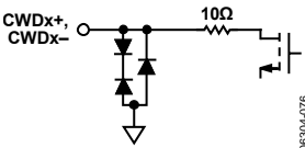
Figure 16. Equivalent CWD Output Circuit
