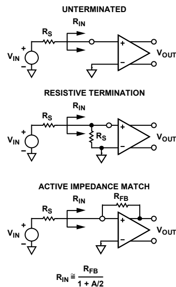
Figure 36. Input Configurations
