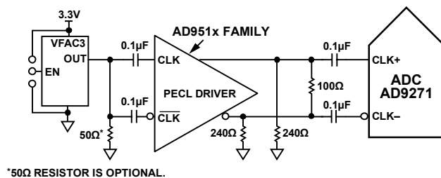
Figure 47. Differential PECL Sample Clock
