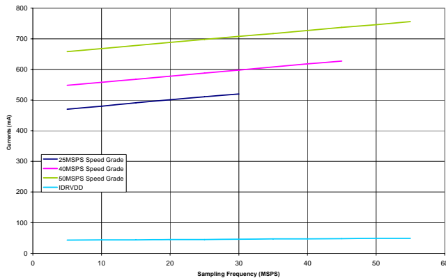
Figure 52. Supply Current vs. f_{\text{SAMPLE}} for f_{\text{IN}} = 7.5 MHz
