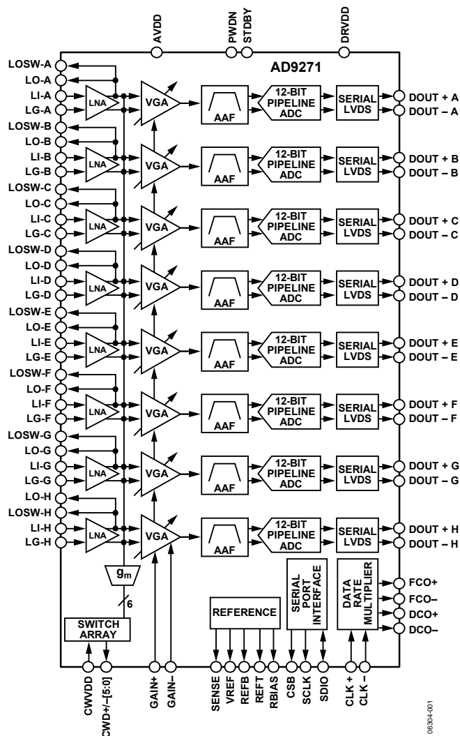
Figure 1. Block Diagram
