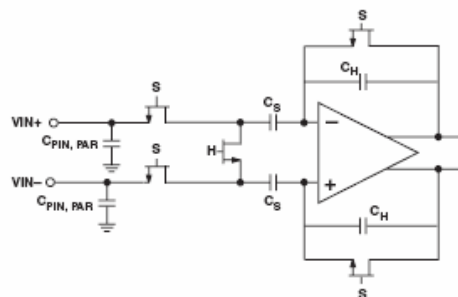
For best dynamic performance, the source impedances driving VIN+ and VIN- should be matched.
