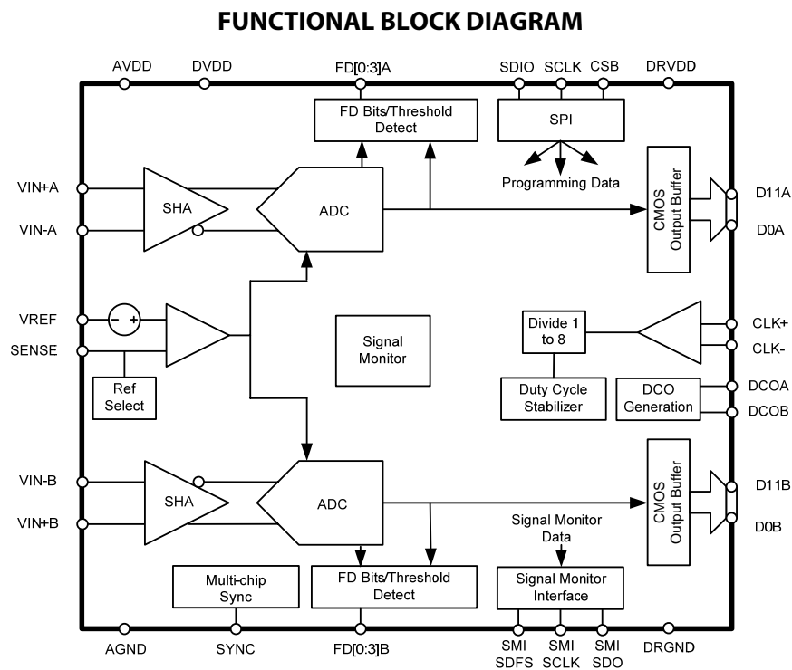
Figure 1. AD9627 Functional Block Diagram
