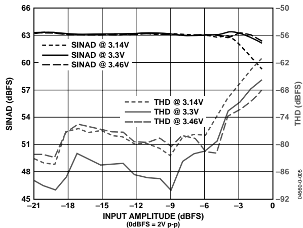
Figure 5. SINAD and THD vs. Input Amplitude and Supply ( f_{\text{IN}} = 8 MHz, \text{LPF } f_{-3\text{dB}} = 26 MHz; R_{\text{xPGA}} = 0 dB)
