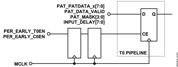
Figure 9. PER_EARLY_T0EN Pipelining
