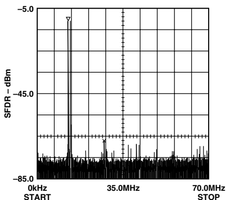
TPC 18. Dual-Tone SFDR @ f_{CLOCK} = 140\text{ MHz} ( f_{OUT1} = 13.5\text{ MHz} , f_{OUT2} = 14.5\text{ MHz} )
