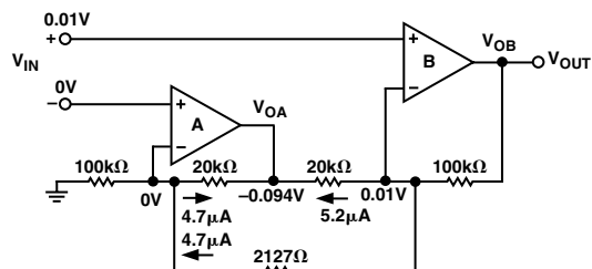
Figure 2. Gain = 100 Instrumentation Amplifier
