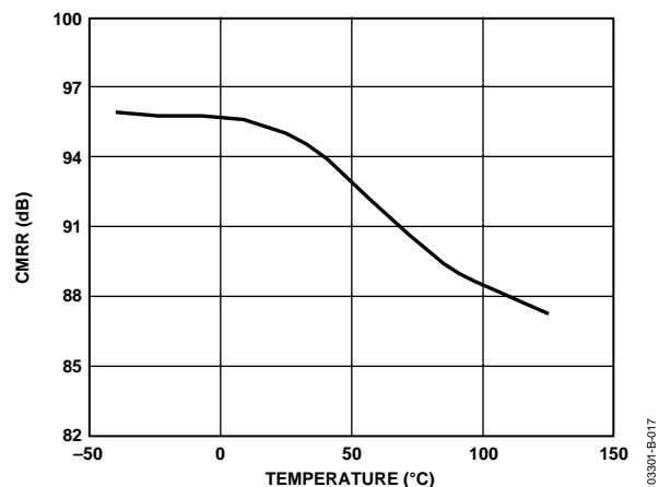
Figure 17. CMRR vs. Temperature
