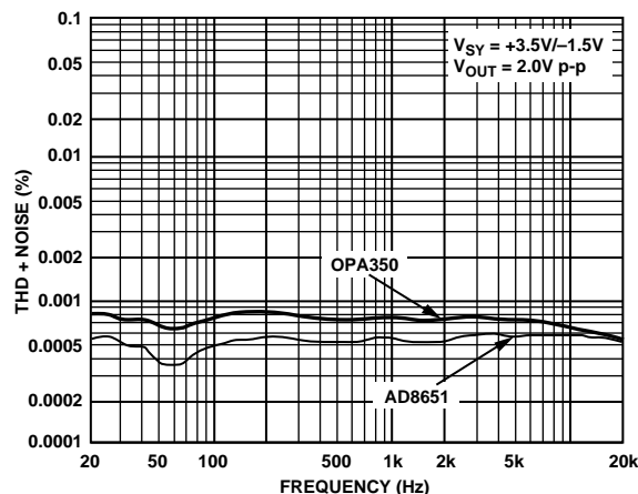
Figure 57. Total Harmonic Distortion
