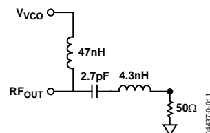
Figure 21. Optimum ADF4360-3 Output Stage
