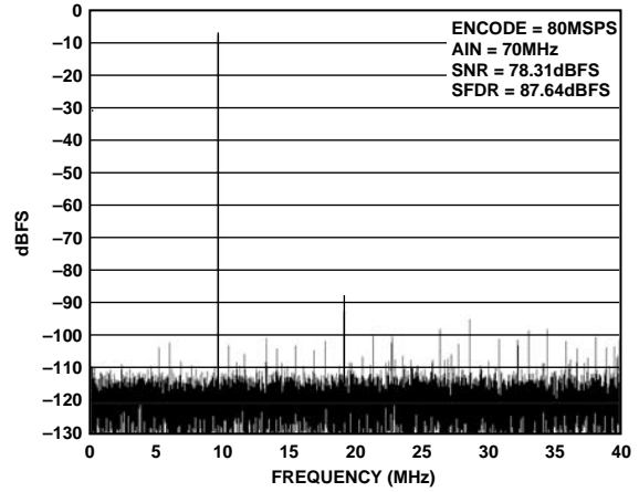
Figure 11. Single-Tone at 70 MHz
