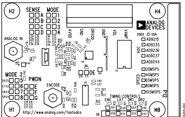
Figure 55. LFCSP Evaluation Board Layout, Primary Silkscreen
