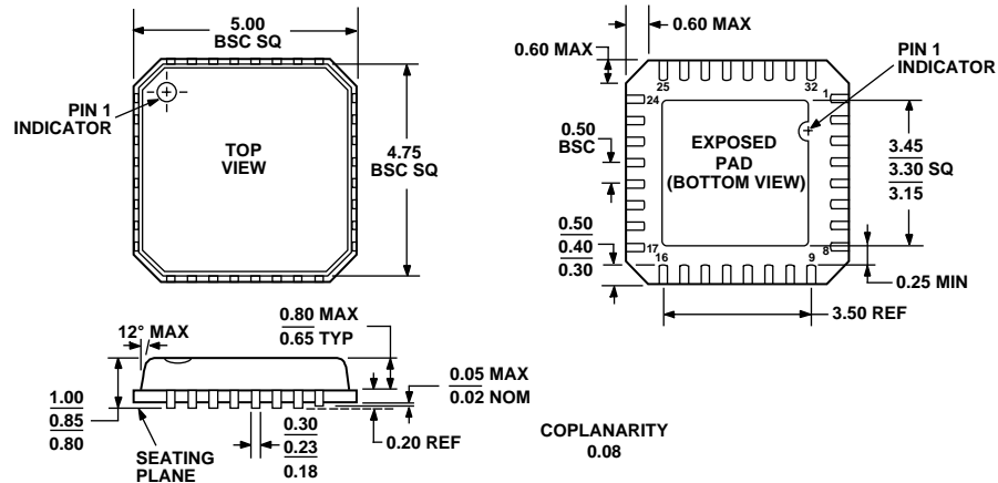
Figure 47. 32-Lead Lead Frame Chip Scale Package [VQ_LFCSP] 5 mm × 5 mm Body, Very Thin Quad (CP-32-3) Dimensions shown in millimeters
