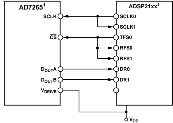
Figure 43. Interfacing the AD7265 to the ADSP218x
