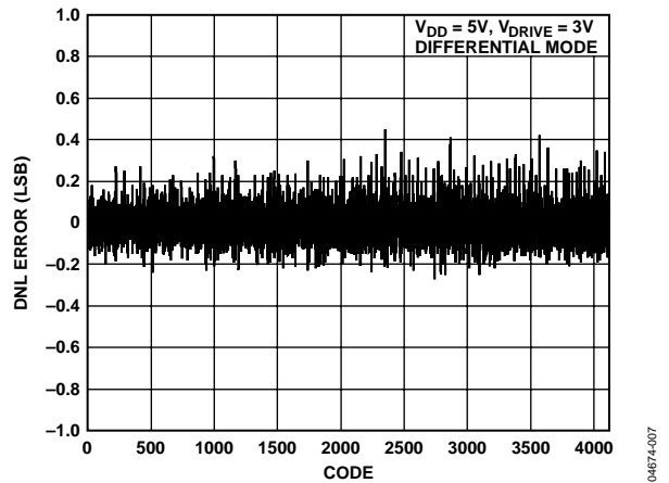
Figure 8. Typical DNL
