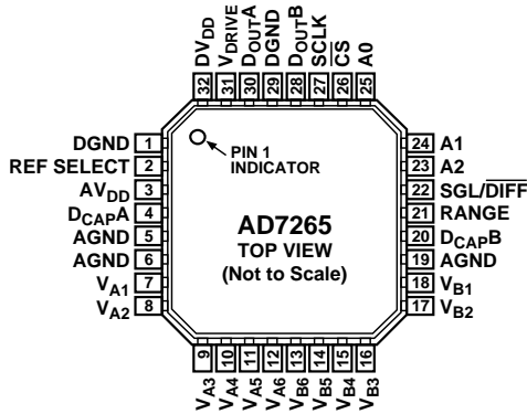
Figure 2. 32-Lead CP-32-3
