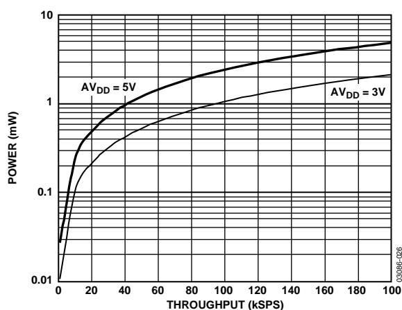
Figure 26. Power vs. Throughput Rate
