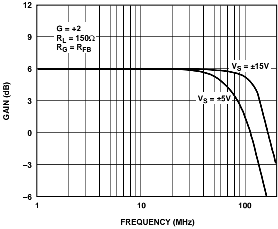
Figure 6. Frequency Response
