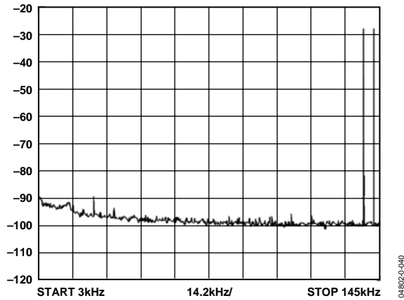
Figure 40. Out-of-Band MTPR
