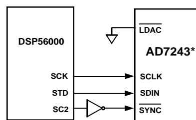
Figure 12. AD7243–DSP56000 Interface
