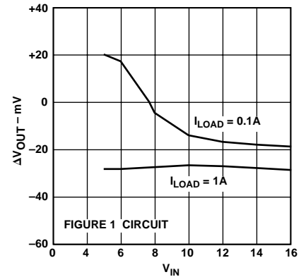
Figure 8. ADP1148-5 Output Voltage Change vs. Input Voltage
