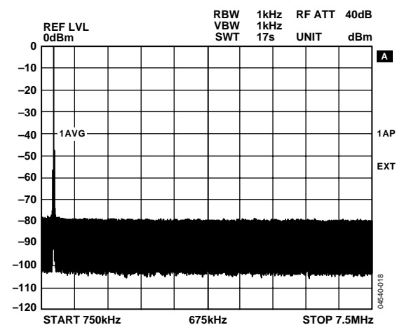
Figure 10. THD @ 400 MSPS and f_{OUT} = 1 MHz (Diplexer Low-Pass Output Showing 0 dBm Fundamental; See Performance Effects of Calibration Section)
