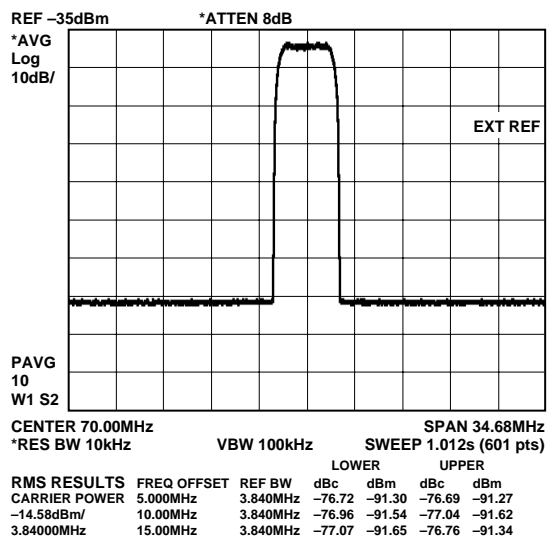
Figure 13. One-Carrier WCDMA @ 400 MSPS f_{OUT} = 70 MHz
