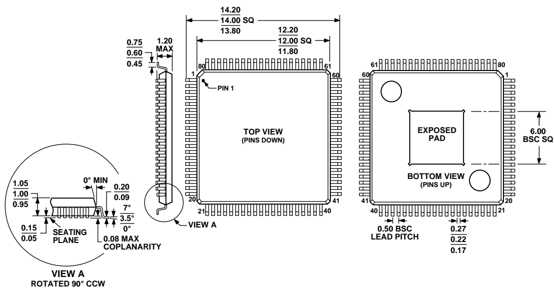
Figure 22. 80-Lead Thin Plastic Quad Flat Package, Exposed Pad [TQFP_EP] (SV-80-1)
