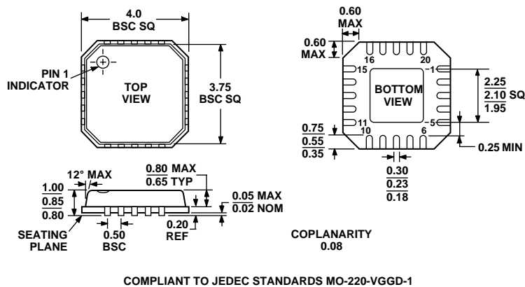
Figure 27. 20-Lead Lead Frame Chip Scale Package [LFCSP] 4 mm × 4 mm Body, (CP-20) Dimensions shown in millimeters
