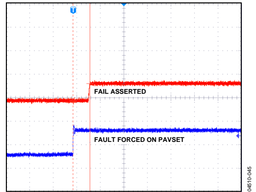
Figure 21. FAIL Assert Time, 1 \mu\text{s/div}
