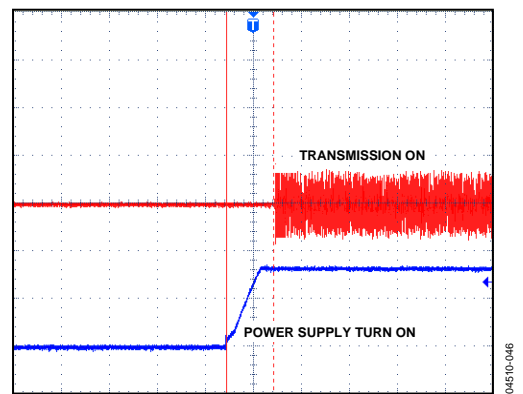
Figure 22. Time to Initialize, Including Reset, 40 \text{ ms/div}
