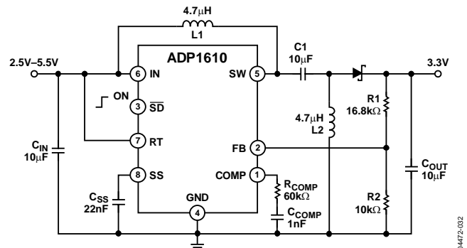
Figure 30. 3.3 V DC-DC Converter
