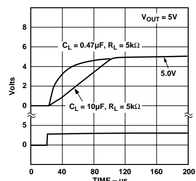
Figure 16. Turn-On
