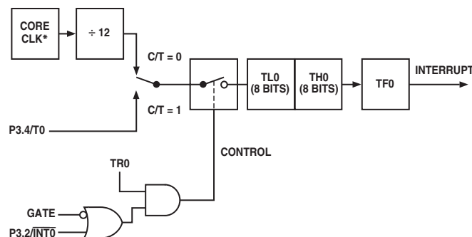
Figure 46. Timer/Counter 0, Mode 1
