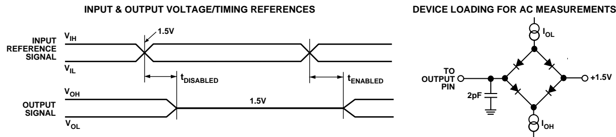
Figure 22. Test Condition Voltage Reference and Device Loading
