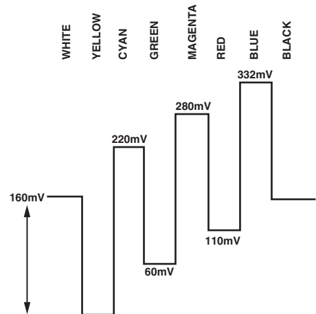
Figure 101. U Levels—PAL
