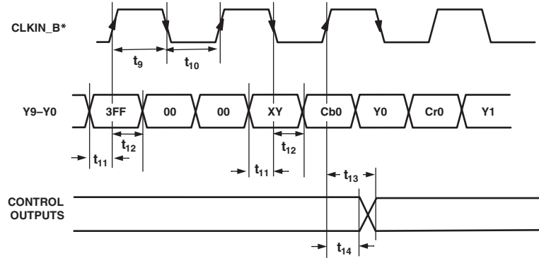
Figure 5. PS 4:2:2 1 × 10-Bit Interleaved at 54 MHz \overline{\text{HSYNC}}/\overline{\text{VSYN}}\overline{\text{C}} Input Mode [Input Mode 111]
