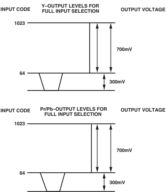
Figure 95. Output Levels for Full Input Selection
