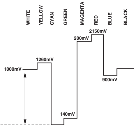
Figure 102. U Levels—NTSC
