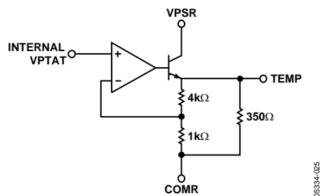
Figure 53. TEMP Interface Simplified Schematic
