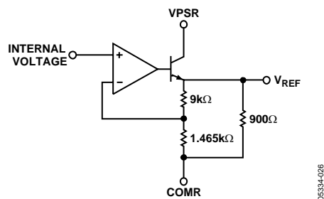
Figure 54. VREF Interface Simplified Schematic
