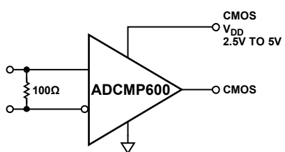
Figure 20. LVDS-to-CMOS Receiver
