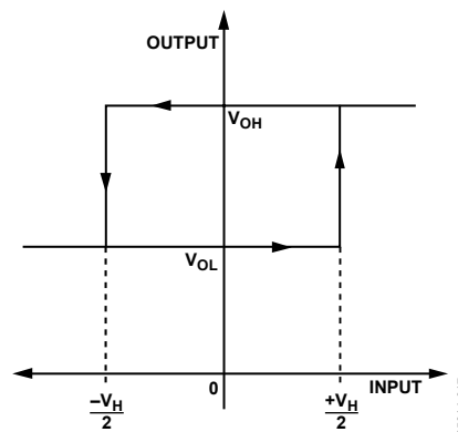
Figure 17. Comparator Hysteresis Transfer Function
