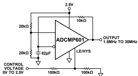
Figure 21. Voltage-Controlled Oscillator
