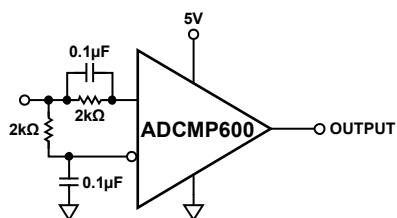
Figure 19. Self-Biased, 50% Slicer
